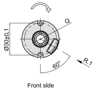
Front side
